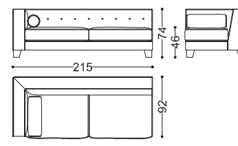
art. 40005/SX - available art. 40005/DX
