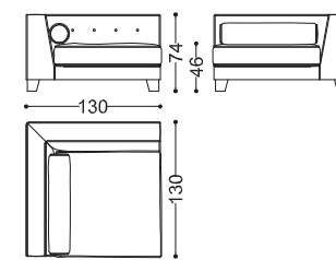
art. 40008 large corner
