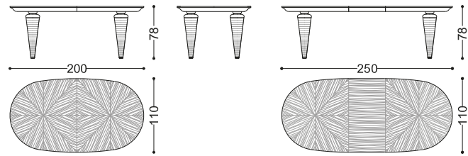
46004/22 FIDELIA oval table
