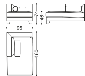
art. 40006/SX - available art. 40006/DX
