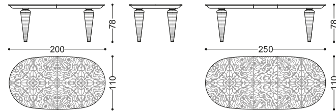
46004/R22 FIDELIA oval table - oak burr top
